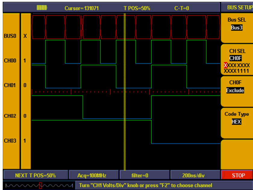
Fig. 93 Bus setting
