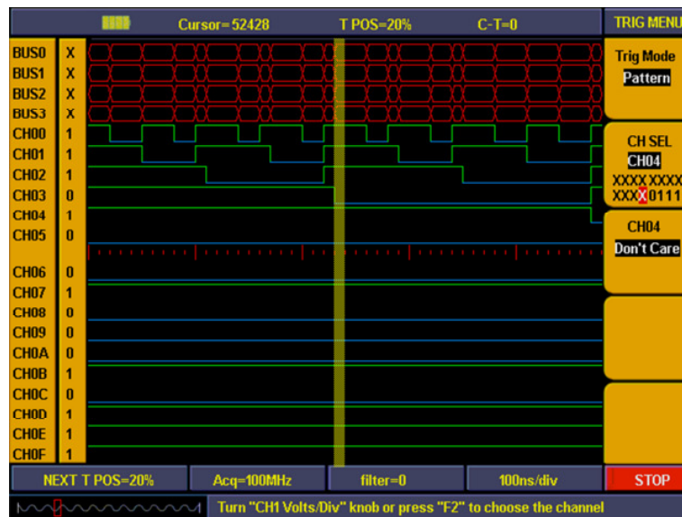
Abb. 82 Pattern-Trigger
