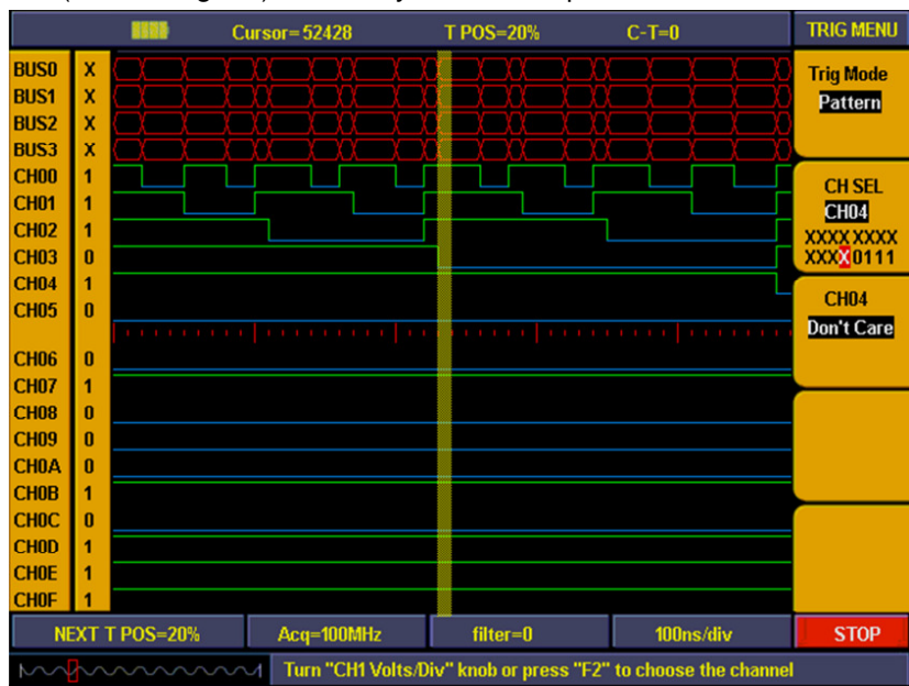
Fig. 81 Pattern trigger
