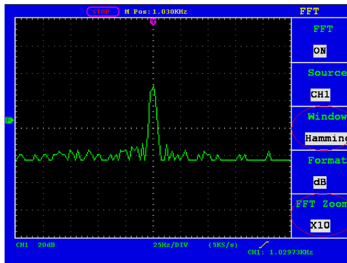
Fig. 28 Hamming window
