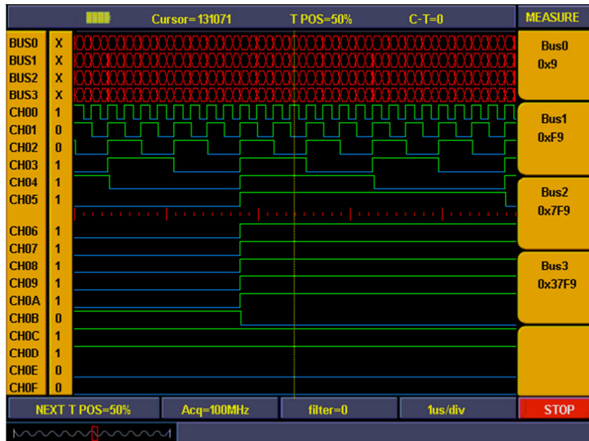
Fig. 94 Bus measurement
