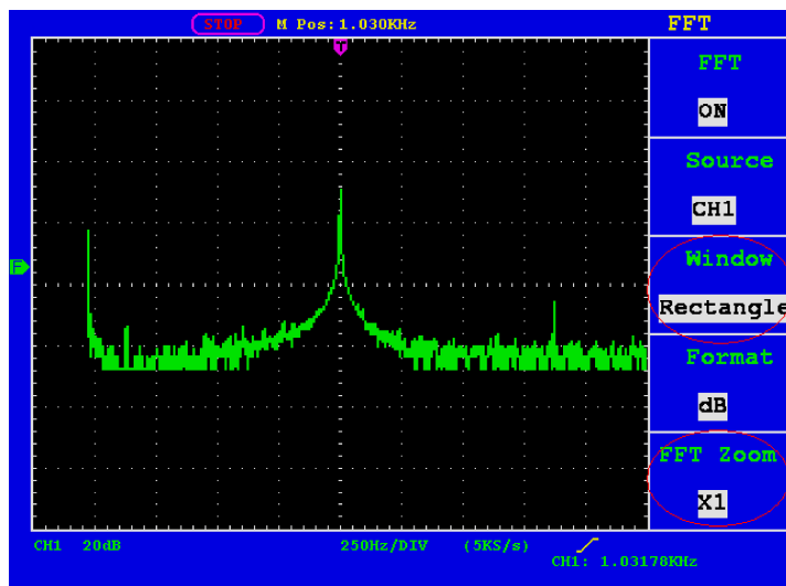
Fig. 29 Rectangle window
