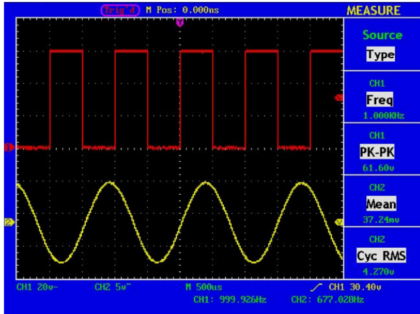
Fig. 65 Automatic Measurement
