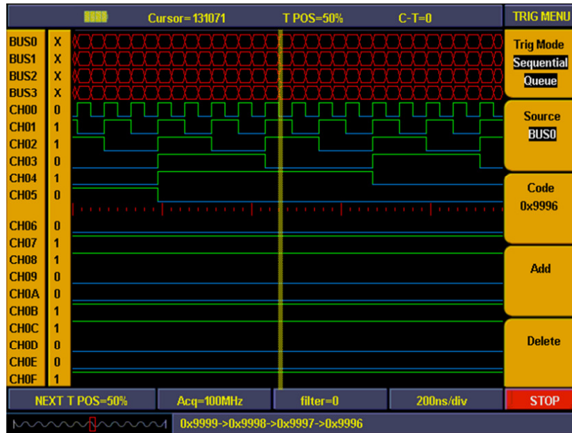
Abb. 84 Sequential Queue-Trigger
