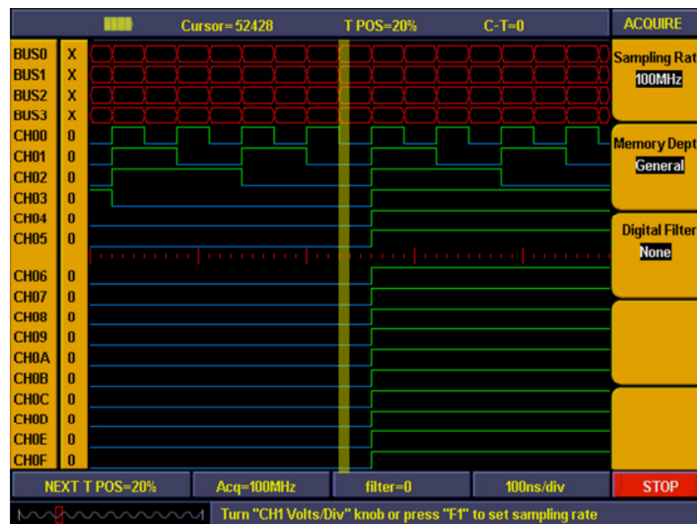
Fig. 75 Sampling setting
