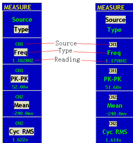
Fig. 64 Measure Menu
