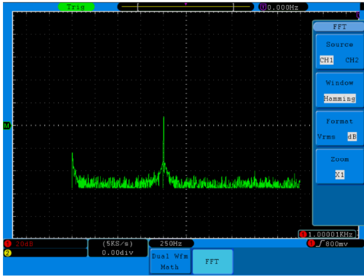
Fig. 21 Hamming window
