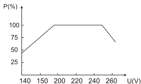
THE POWER CURVE OF OUTPUT
